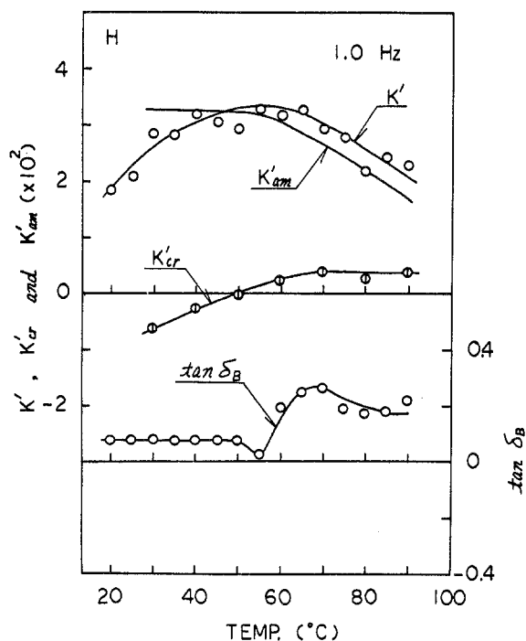
Figure 9. The variation of the measured strain-optical coefficient K' , the calculated crystalline and amorphous contributions, K'_{cr} and K'_{am} , and the tangent of the birefringence-strain phase angle with temperature at a frequency of 1 Hz for heat-treated low-density polyethylene.
